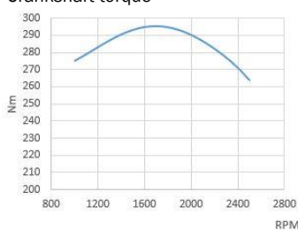
Crankshaft torque
