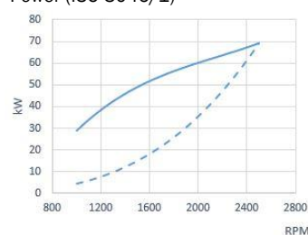
Power (ISO 3046/1)
