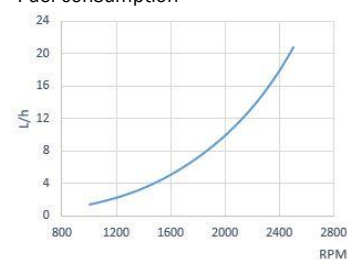
Fuel consumption
