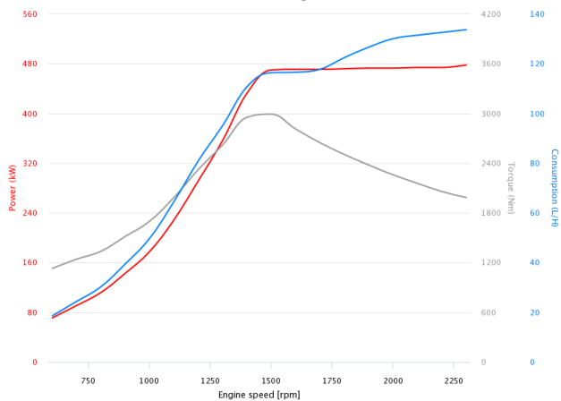
C16 1000 - Rating C: 478 kW
