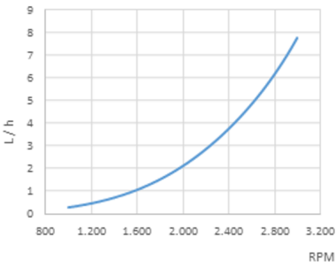
Fuel consumption
