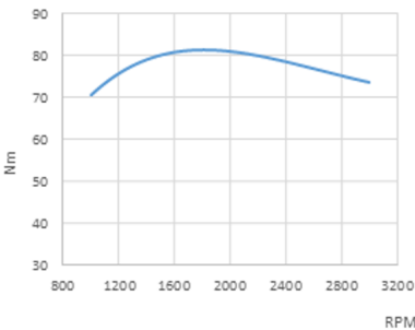
Crankshaft torque
